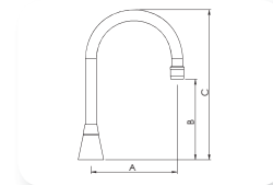
1/4 turn ceramic disc (LFQ)
