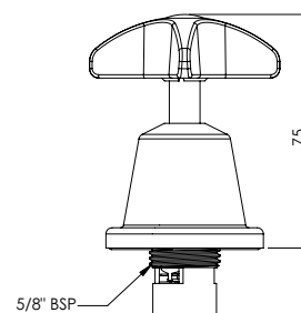
VPQ391 CERAMIC DISC
