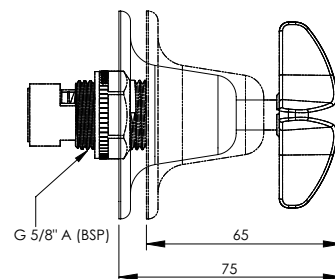
VPQ391 CERAMIC DISC
