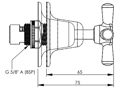
INQ308 CERAMIC DISC
