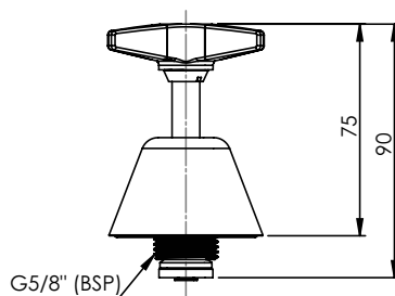
PZ391 JUMPER VALVE
