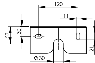
BRACKET MOUNTING DETAILS
